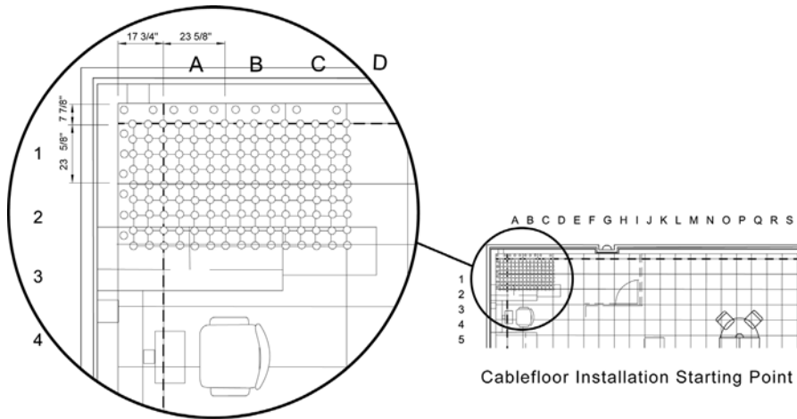
Location & Dimension for Chalk Lines to Start Installation
